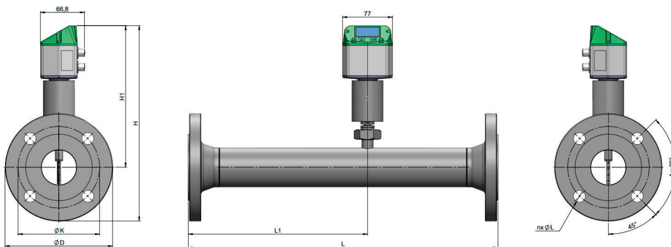
VD 520 - with flange (Material stainless steel: 1.4404)
