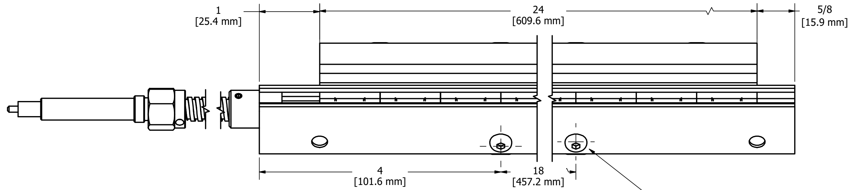
FRONT VIEW
