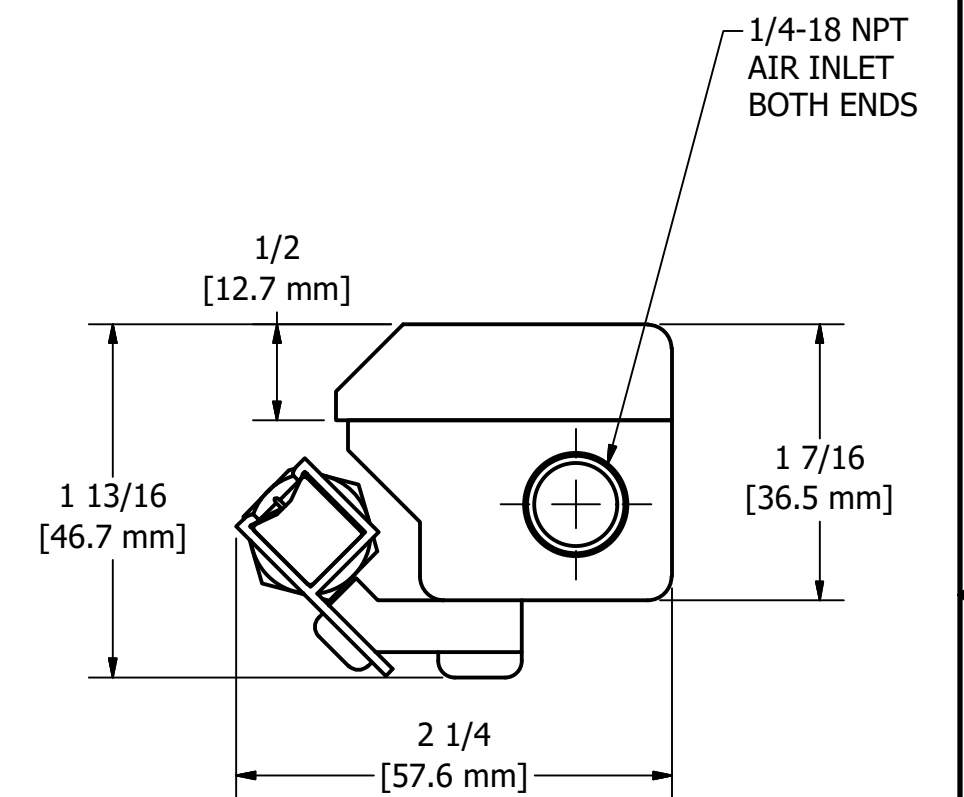
END VIEW
