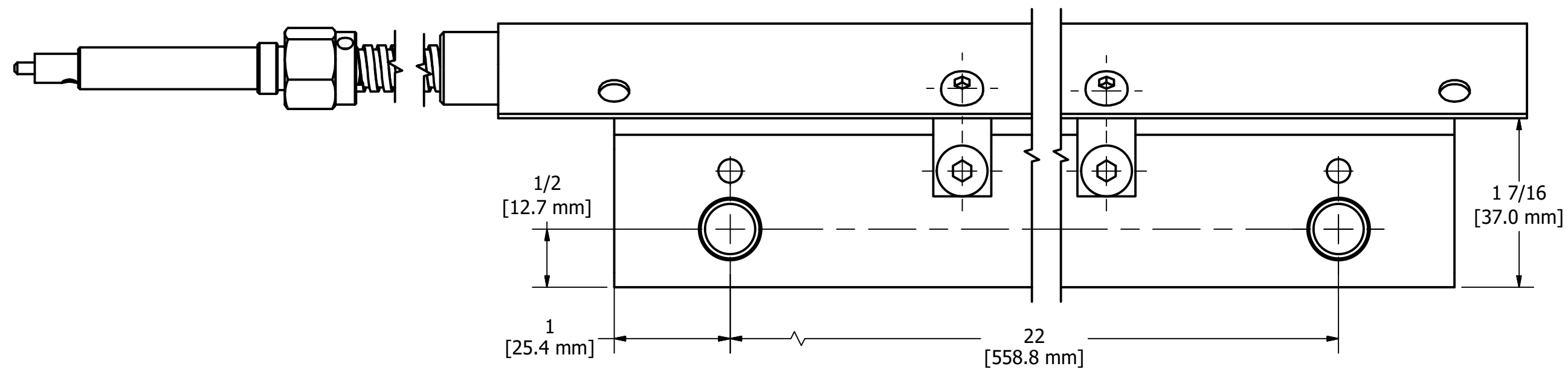
BOTTOM VIEW
