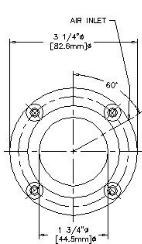
END VIEW
