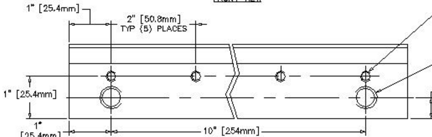
BOTTOM VIEW
