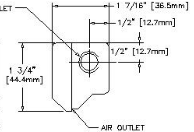
END VIEW
