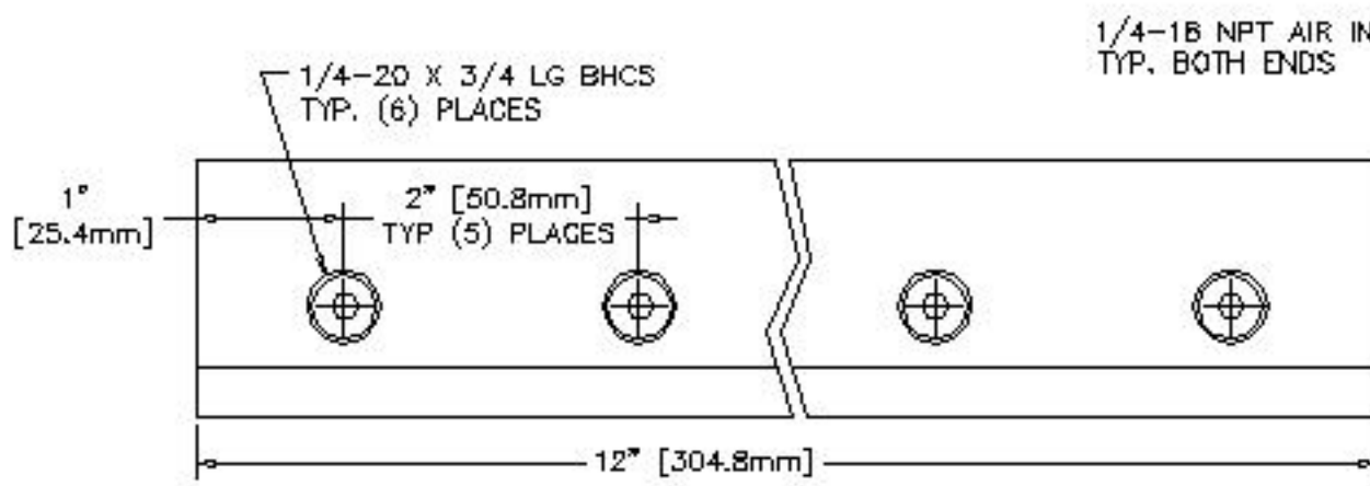
TOP VIEW
