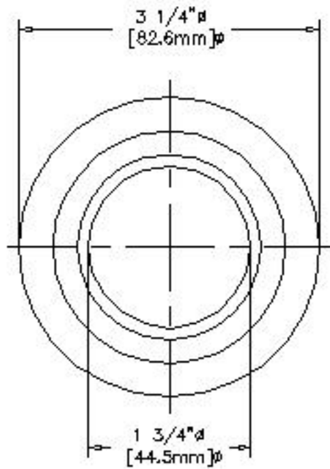
END VIEW
