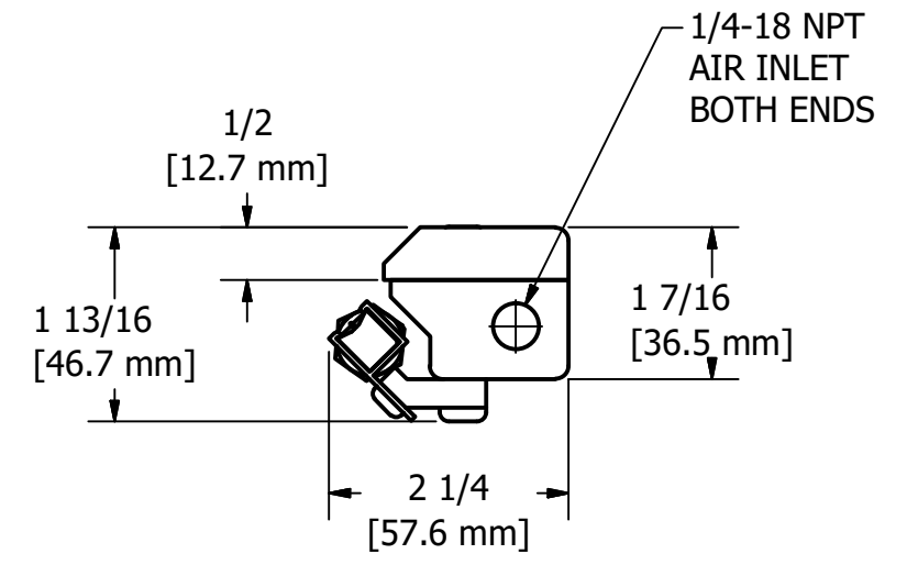
END VIEW
