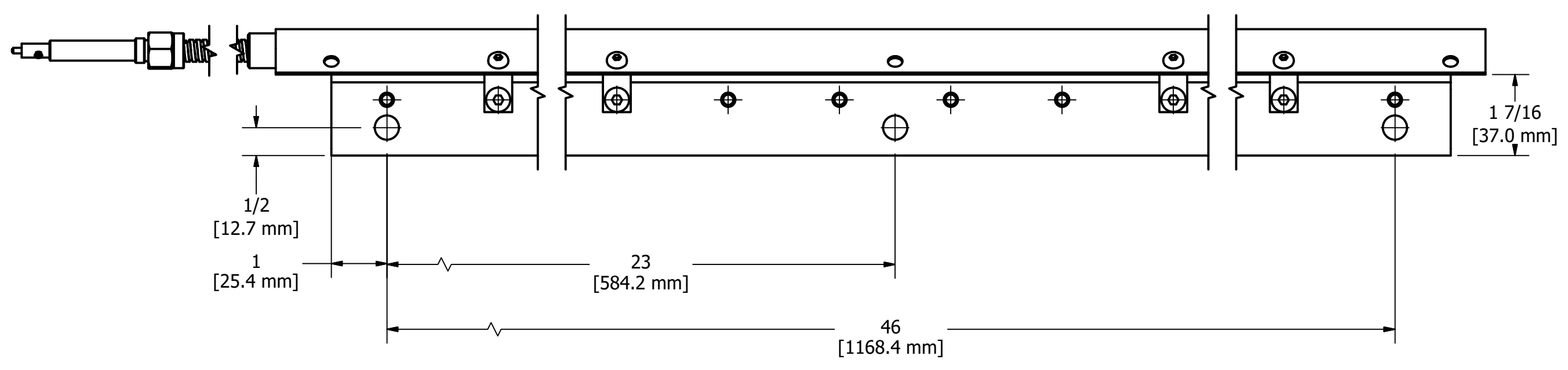
BOTTOM VIEW
