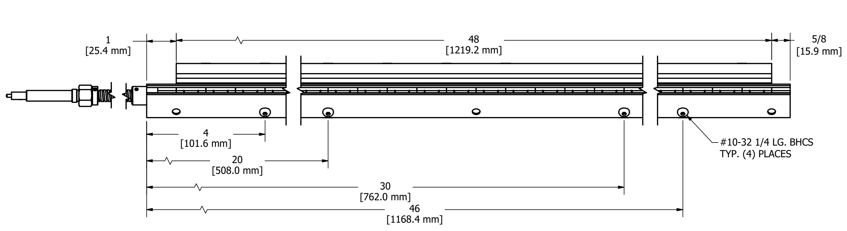
FRONT VIEW
