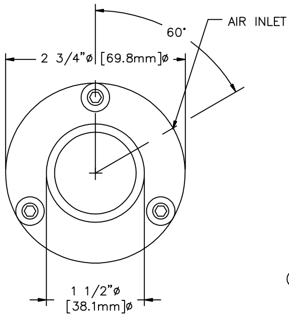
END VIEW
