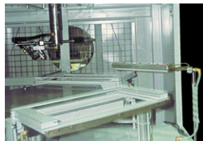
A Model 7212 12" (305mm) Standard Ion Air Knife System cleans metal frames prior to powder coating.
