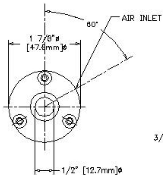
END VIEW
