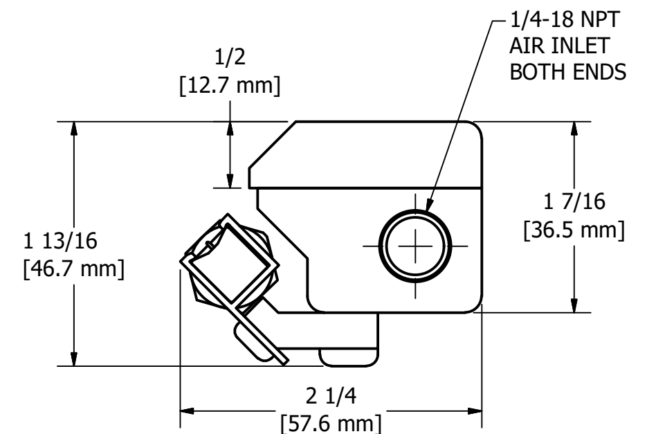
END VIEW
