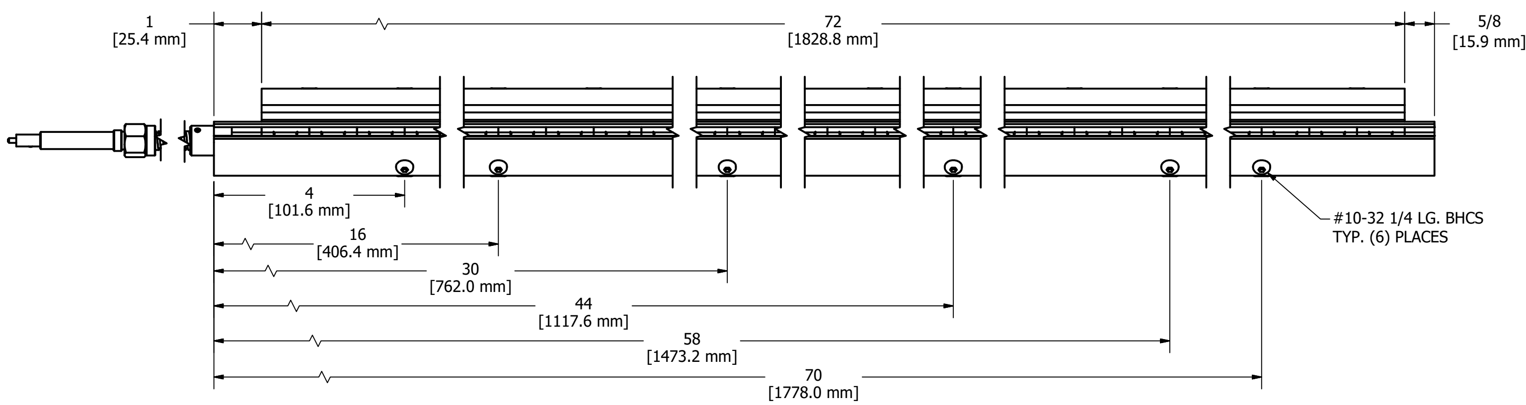
FRONT VIEW
