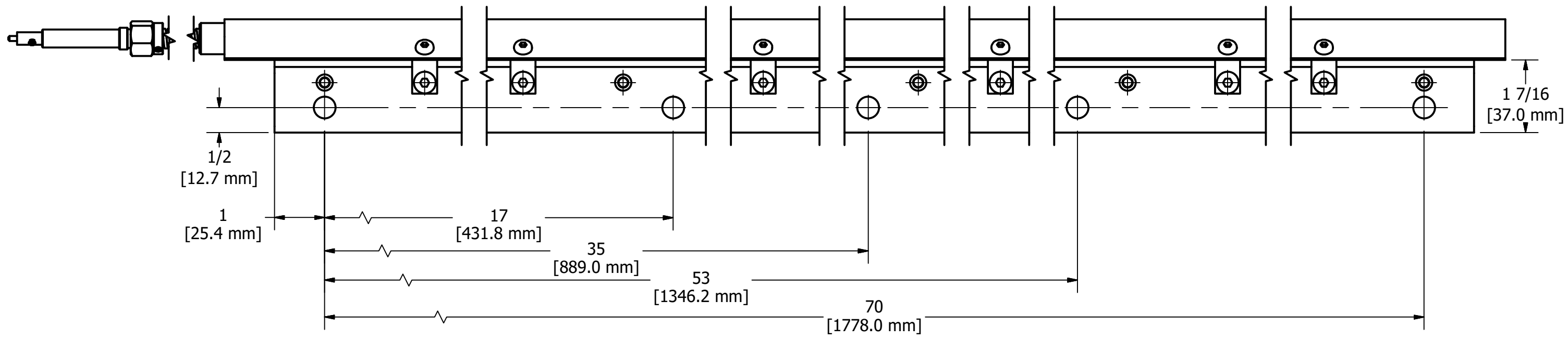
BOTTOM VIEW
