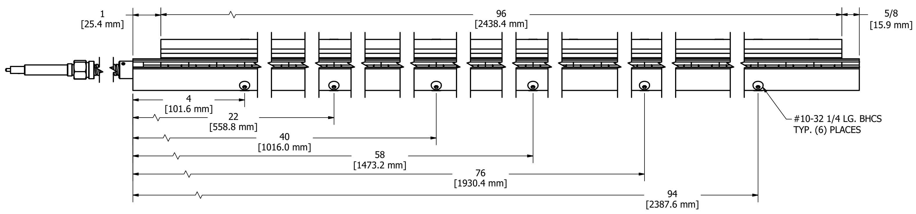
FRONT VIEW
