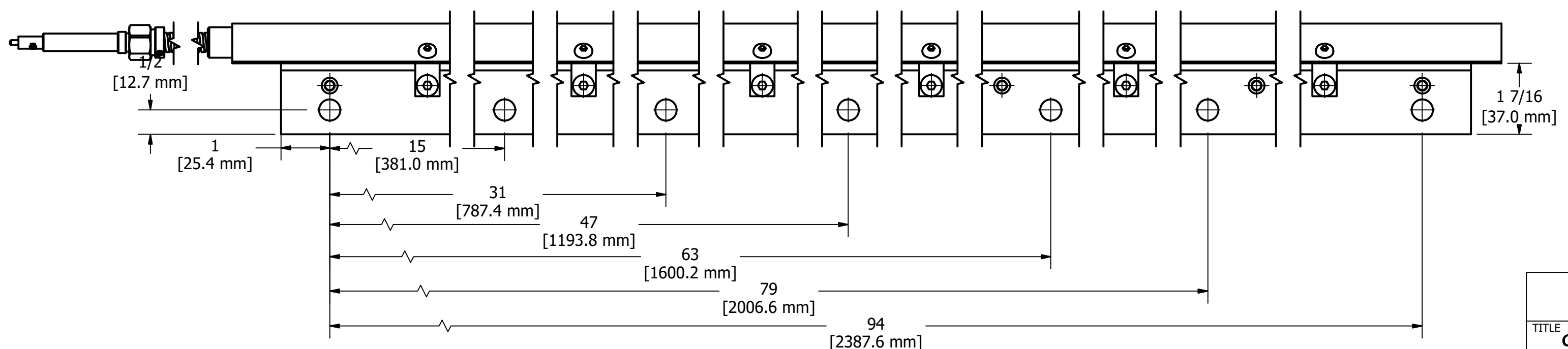
BOTTOM VIEW
