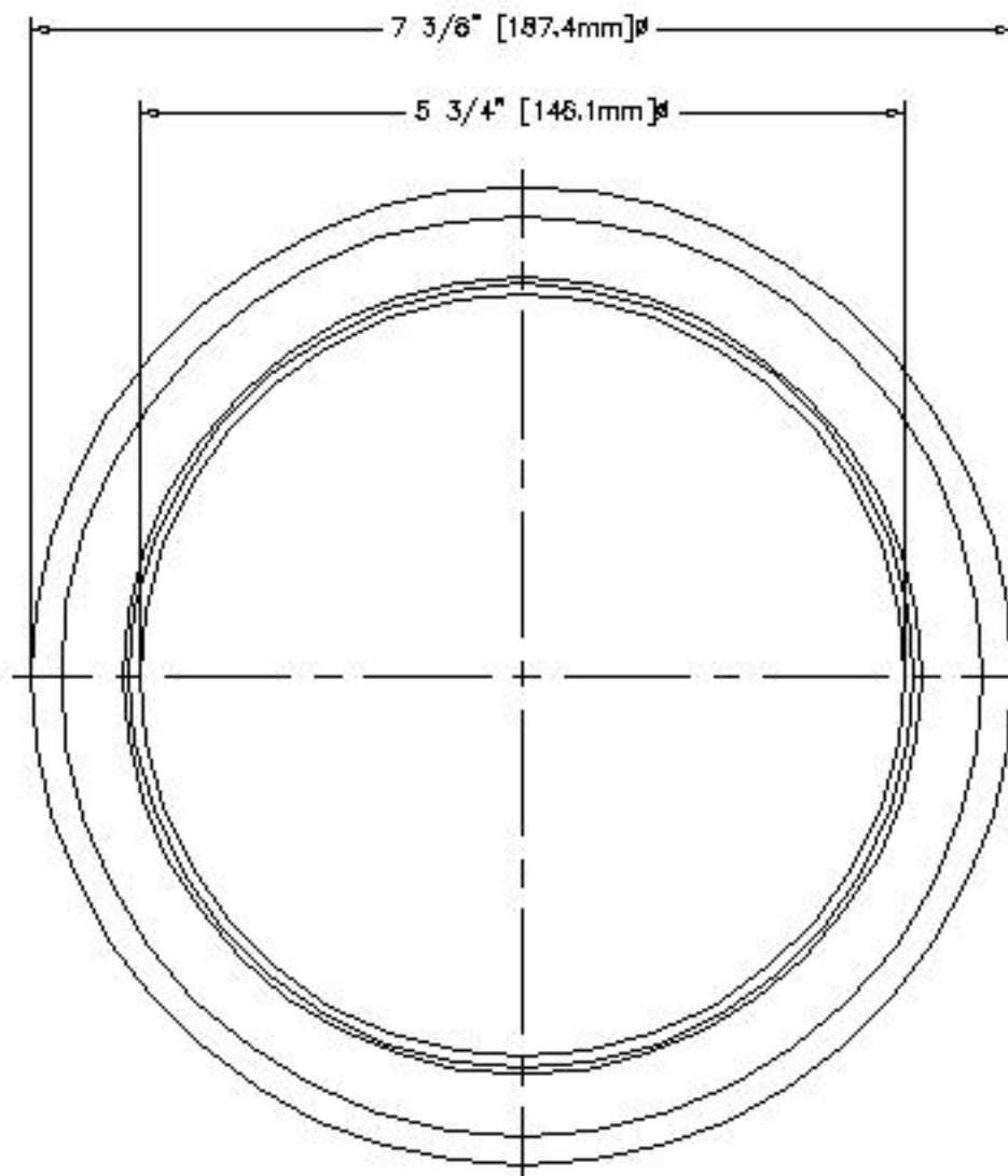
END VIEW
