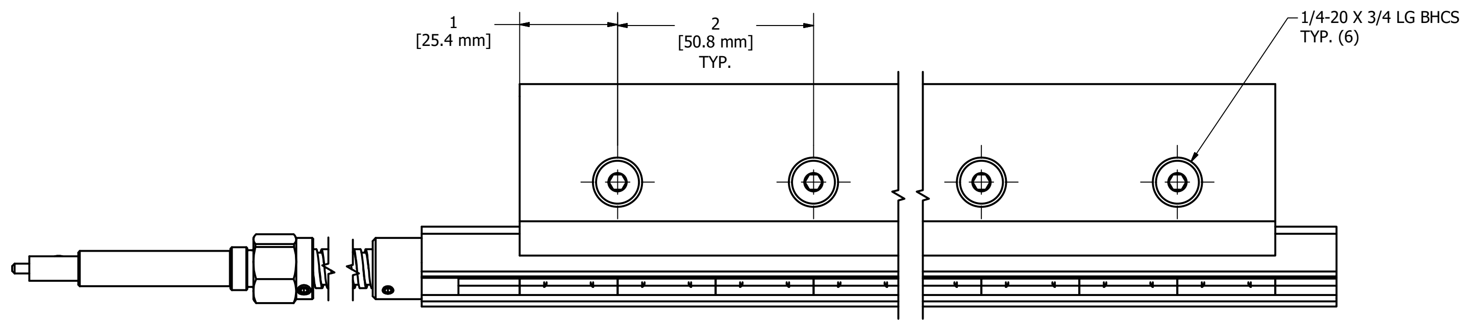
TOP VIEW
