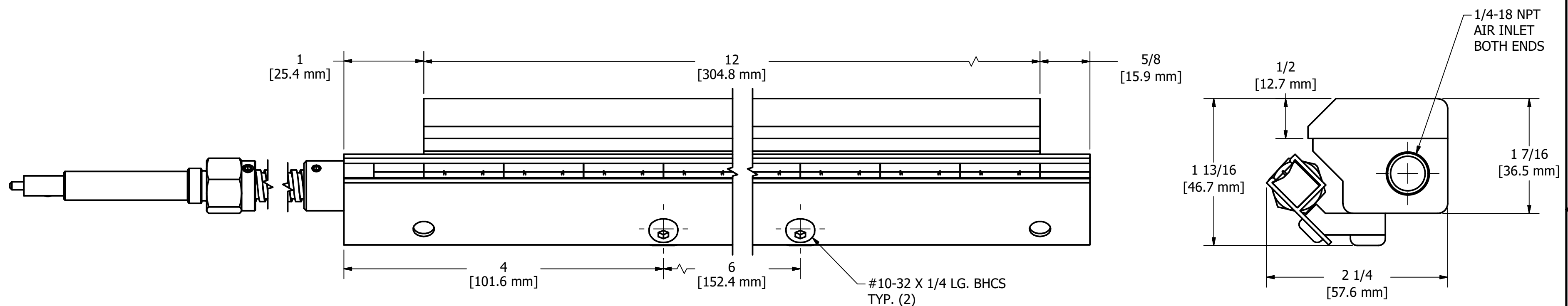
FRONT VIEW
