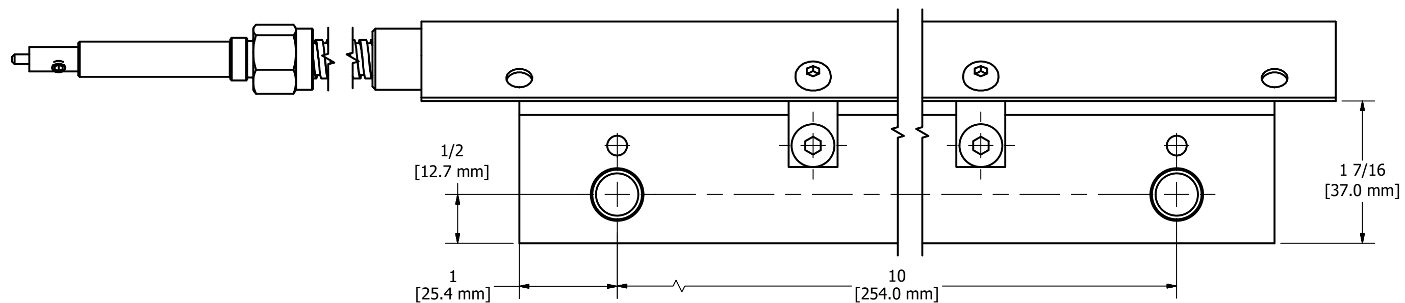
BOTTOM VIEW
