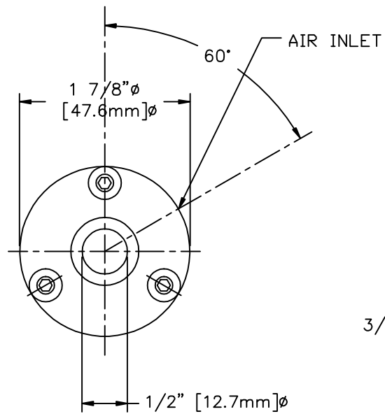
END VIEW
