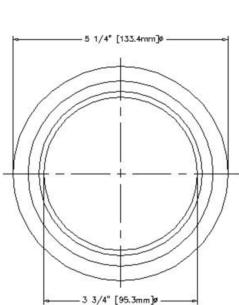
END VIEW
