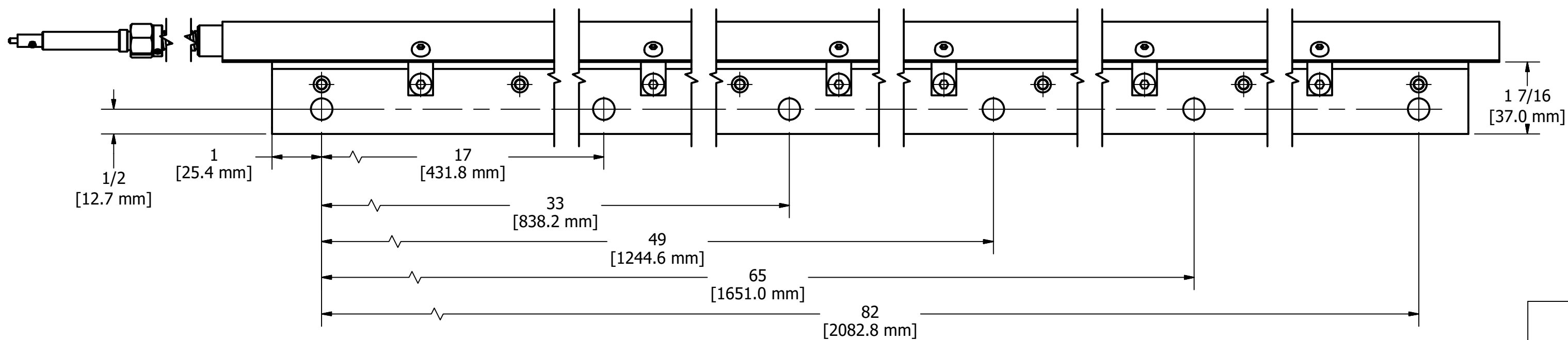
BOTTOM VIEW
